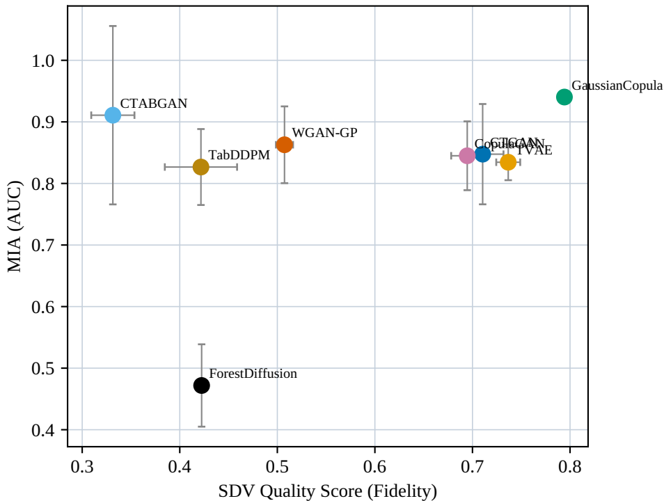
Alzheimer's: SDV Quality Score (Fidelity) vs MIA (AUC)
